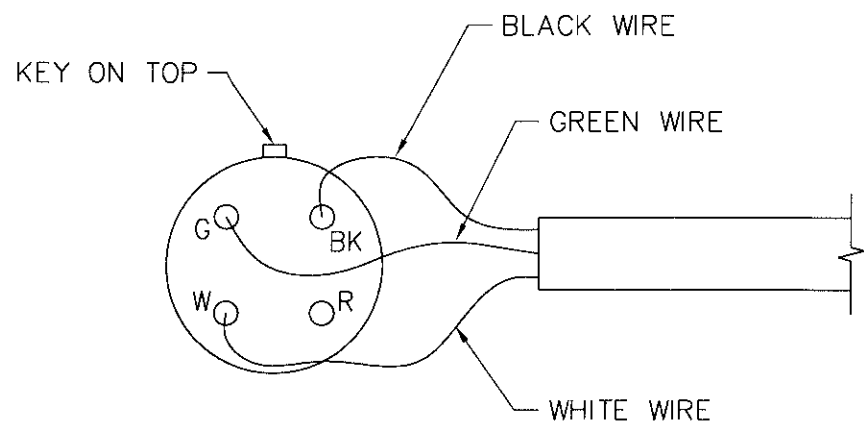
VIEW FROM BACK OF PLUG
